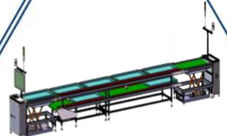
高压线束流水线 (升降回转--皮带式) High-Voltage Conveyor Line (Lifting-Belt Type)
